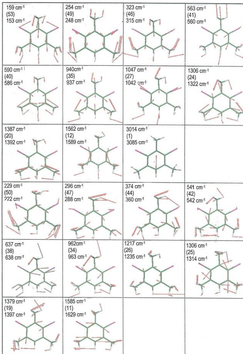
Fig. 7. Illustration of the atomic displacements for the twenty one “skeleton” in-plane vibrational modes (from DFT calculations): the first number at the top of each small figure corresponds to the frequency of an experimental observation (Raman or IR), the second (in parentheses) corresponds to the numbering from the highest frequency to the lowest, and the third number is the calculated anharmonic frequency.
