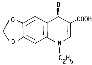
Oxolinic acid
