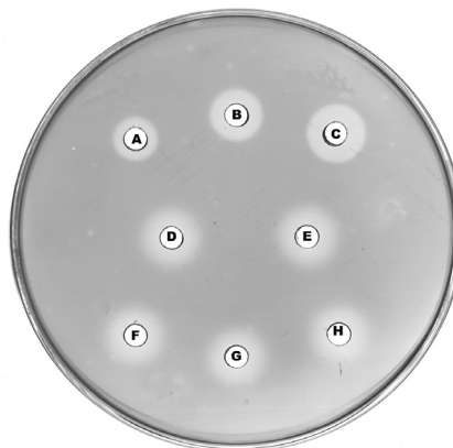
Figure 1. Plate diffusion for milk and donkey's milk fermented beverage. Lysozyme determination: wells A, B, C lysozyme standard solutions (1, 2, 4 ppm); wells D, E diluted milk, respectively before and after pasteurization at 63 °C for 30 min; wells F, G, H diluted fermented beverage 7, 15 and 30 d after inoculation.
