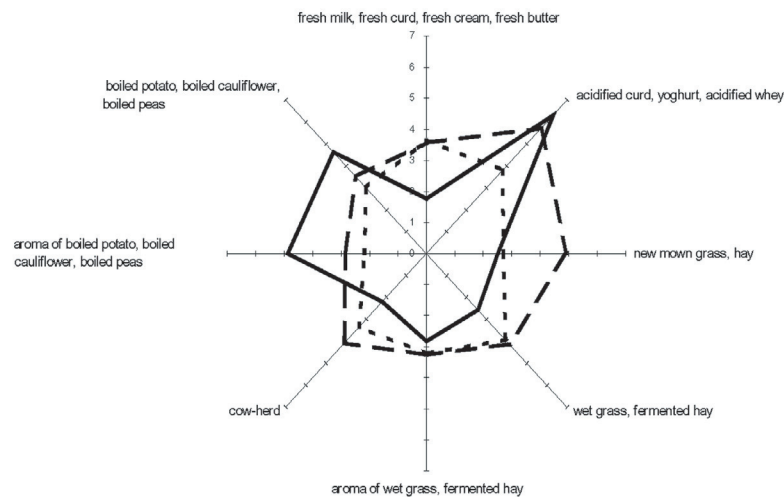
Figure 3. Presentation of the 8 descriptors (average of the evaluation by 15 consumers), which allows the differentiation of beverages fermented with the three strains (— L. rhamnosus AT 194, --- L. rhamnosus CLT 2/2, ..... L. casei LC 88).
