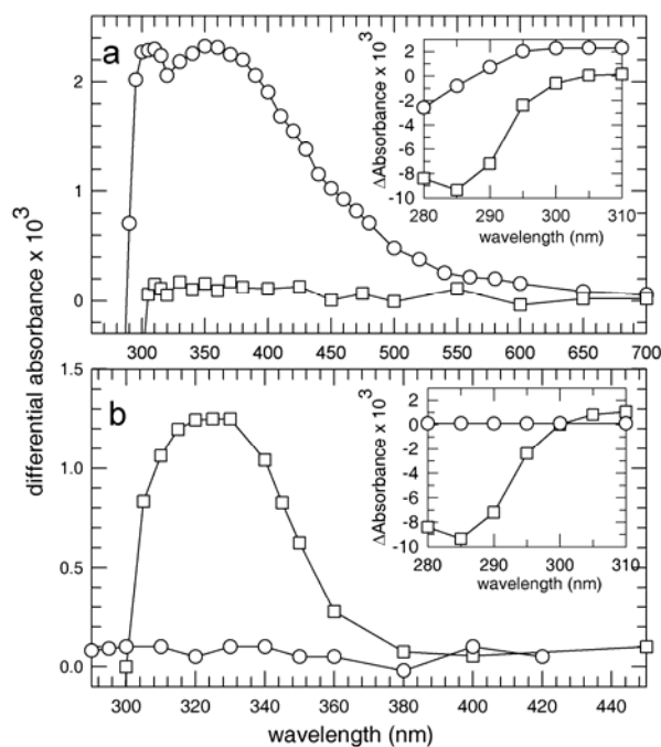
Figure 2. Transient absorption spectra recorded at 200 ns (a) and 10 ms for TMP (circles) and at (dT) 20 (squares). Excitation density at 266 nm: 1.2 \text{ MW/cm}^2 .
