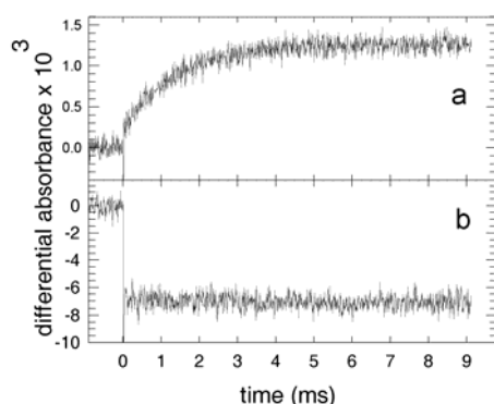
Figure 3 Transient signals obtained for (dT)_{20} at 325 nm (a) and 290 nm (b). Excitation density at 266 nm: 1.2 MW/cm 2 . None of the signals is affected when oxygen is bubbled in the solution.
