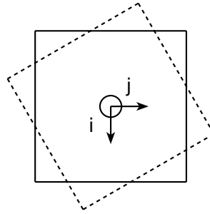
Fig. 7 Composite figure associated to D_4 \cap rD_4r^t where r = \mathbf{Q}\left(\mathbf{k}; \frac{\pi}{3}\right)
