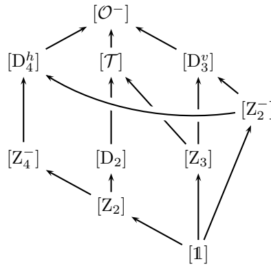
Fig. 8 Partially ordered set of conjugacy classes of closed subgroups of O^-
