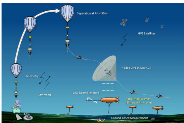
Figure 13: Diagram of D-SEND #2 test planned for 2013.
