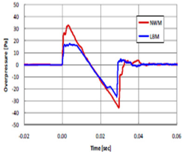
Figure 11: Contrasting sonic boom signatures recorded with NWM and LBM test bodies.
