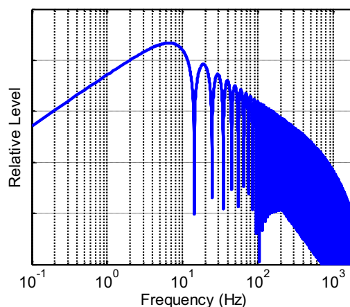
Figure 1: Acoustic content of a sonic boom.
