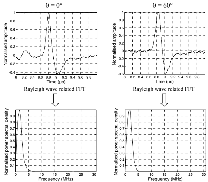
Figure 4: normal displacement after transmission by the slot and associated spectra ( \theta = 0^\circ and \theta = 60^\circ )
