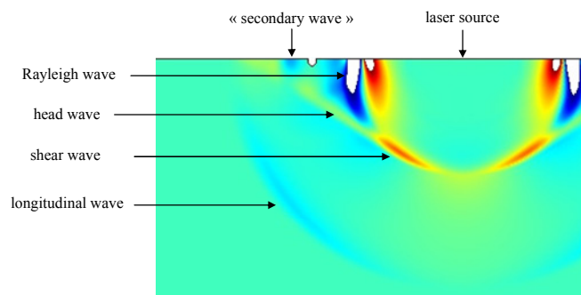
Figure 10: calculated normal displacement in aluminium (0,5 \mu\text{s} after the laser shot)
