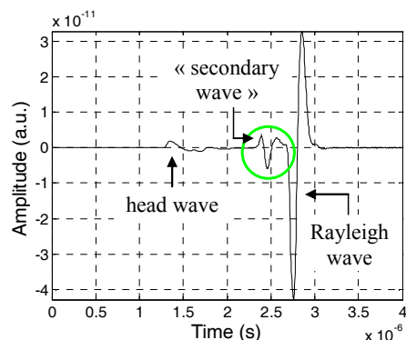
Figure 11: calculated normal displacement as a function of time for d_{GS} = 2\text{ mm} , d_{SD} = 6\text{ mm}
