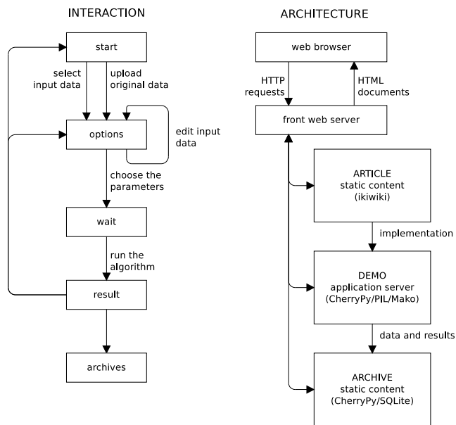
Fig. 1. Workflow and design of the web demo system.
