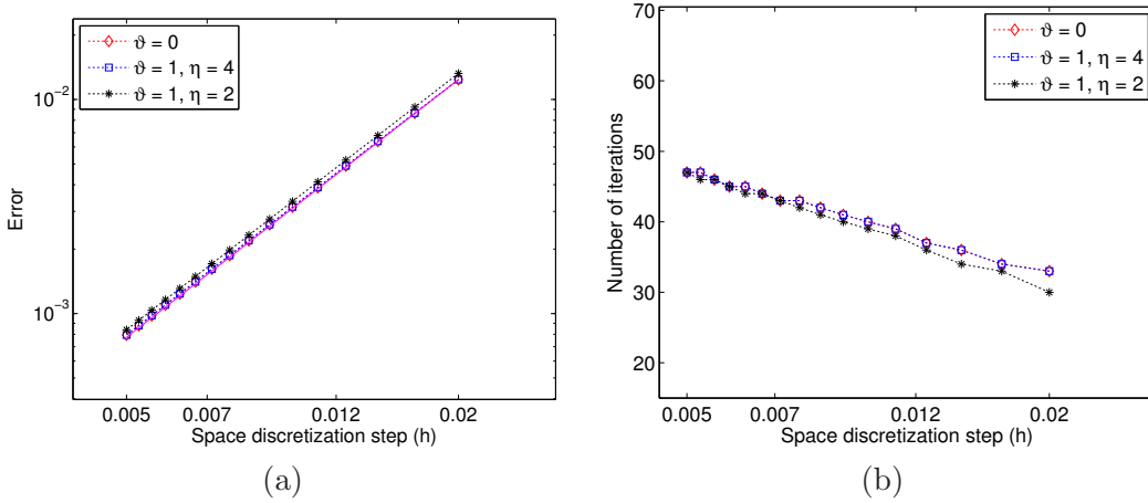
Figure 2: (a) Error for a fixed period T = \frac{\pi}{2} and for values of h distributed between 1/200 and 1/50 . (b) The number of iterations necessary to achieve a precision \epsilon = h^3 in the fixed point algorithm for T = \frac{\pi}{2} and values of h distributed between 1/200 and 1/50 .
