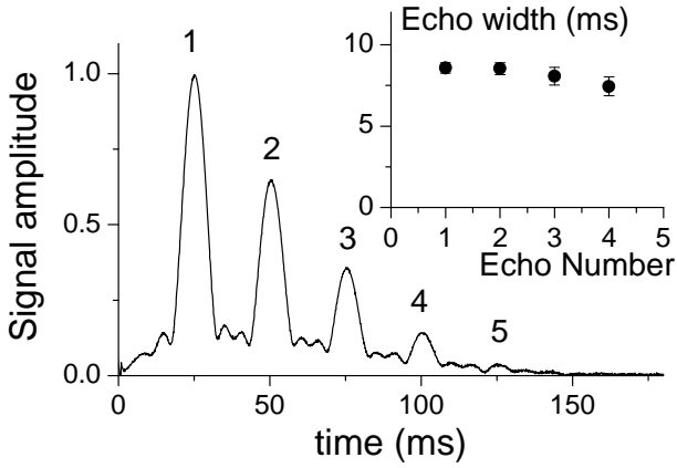
Figure 3: Time-domain variation of signal amplitude obtained with hyperpolarized ^3\text{He} and a constant gradient for \tau = 24.6 ms and f_{\text{dip}} = 5.5 Hz. The diffusion coefficient of ^3\text{He} was 50 times larger than that of ^{129}\text{Xe} , which impeded the observation of more numerous echoes. The inset displays the observation of more numerous echoes. The inset displays the echo widths (FWHM) of the first echoes; they do not increase with echo number, in contrast to those of Fig. 2.
