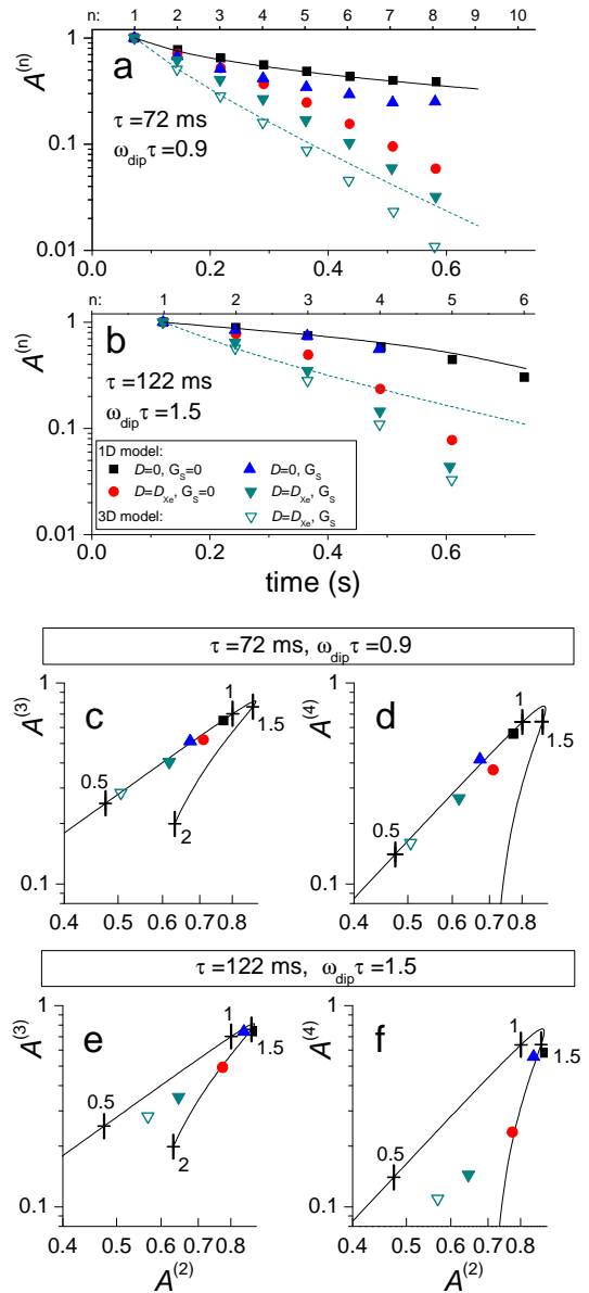
Figure 4: Results of lattice simulations with a 1D model (solid symbols) without or with slice selection G_S and diffusion attenuation D_{\text{Xe}} (see legend in plot b), or a full 3D model with G_S and D_{\text{Xe}} (open triangles). a, b: Reduced echo amplitudes for f_{\text{dip}}=2 Hz and different inter echo times. The solid and dotted lines interpolate values of Eq. 9 at times n\tau for the nominal \omega_{\text{dip}}\tau value and an appropriately smaller \omega_{\text{id.}}\tau value, respectively (see text). c, d (resp. e, f): Reduced amplitudes of the third and fourth echoes in a (resp. b), plotted as functions of the reduced amplitudes A^{(2)} . The solid lines are the ideal case amplitudes of Eq. 9, and the labeled + symbols correspond to the indicated values of \omega_{\text{dip}}\tau .
