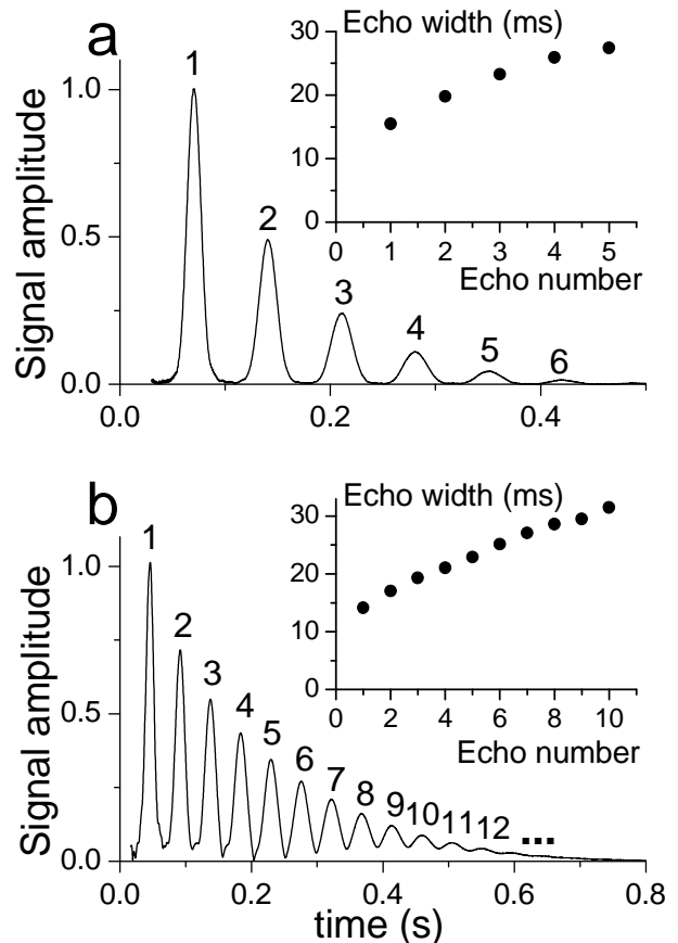
Figure 2: Time-domain variations of signal amplitudes obtained with the pulse sequence of Fig. 1 and dissolved laser-polarized xenon. a: For an inter-echo time \tau = 70 ms and f_{\text{dip}} = 3.1 Hz, a series of Gaussian-shaped echoes is observed. b: A larger number of echoes is obtained with \tau = 45 ms and f_{\text{dip}} = 9 Hz. The insets display the corresponding echo widths (FWHM).
