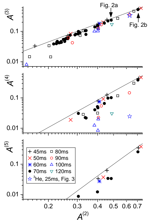
Figure 5: Experimental reduced echo amplitudes A^{(3)} to A^{(5)} (top to bottom) are plotted as functions of A^{(2)} for various \tau (symbols, see legend). The lines are the upper branches ( \omega_{\text{dip}}\tau < 1.5 ) of the corresponding ideal echo amplitudes A_{\text{id.}}^{(n)} (Eq. 9). The data from Fig. 2a ( \omega_{\text{dip}}^{\text{exp}}\tau = 1.4 ) and Fig. 2b ( \omega_{\text{dip}}^{\text{exp}}\tau = 2.5 ) are indicated by the labeled arrows.
