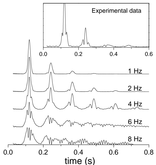
Figure 6: Main plot: numerical 3D lattice simulations of the variation of the echo pattern as a function of f_{\text{dip}} for \tau = 120 ms (with slice-selection and taking into account xenon diffusion). Inset: experimental result with a dissolved laser-polarized xenon sample ( f_{\text{dip}} = 9 Hz). The vertical scale is chosen so as to better visualize the altered echo shapes.
