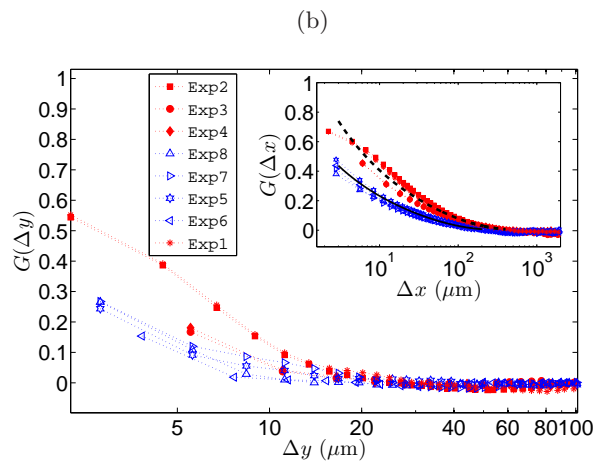
FIG. 7. (a) Time correlation functions collapsed onto each other according to a power law with an exponential cutoff G(\Delta t) = A\Delta t^{-\tau_t} \exp(-\Delta t/t^*) . The exponent is \tau_t \approx 0.43 . Inset shows the scaling between the crossover correlation time and average propagation velocity t^* \approx 7.1 \mu\text{m}/\langle v \rangle . (b) Space correlation function G(\Delta y) with logarithmic \Delta y -axis. Consistently with (a) and Eq. (7), the local velocities become uncorrelated after only a short distance ( \sim 10 - 20 \mu\text{m} ) in the y -direction. Correlation functions from experiments performed on sample #2 and #1 have filled and open markers respectively. To some extent we see also here grouping of experiments from the same sample. The difference is however not as clear as for the spatial correlations along the transverse x -axis (subparallel to the fronts), on the inset showing G(\Delta x) with logarithmic x -axis. The reason might be that the drop to zero correlation occurs close to the resolution scale for G(\Delta y) .
