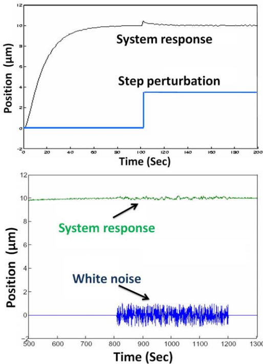
Fig. 12. Step responses with robustified PI controller in presence of (a) step perturbation (b) white noise.
