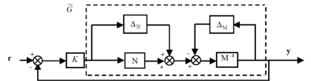
Fig. 4. Coprime factor robust stabilization problem.
