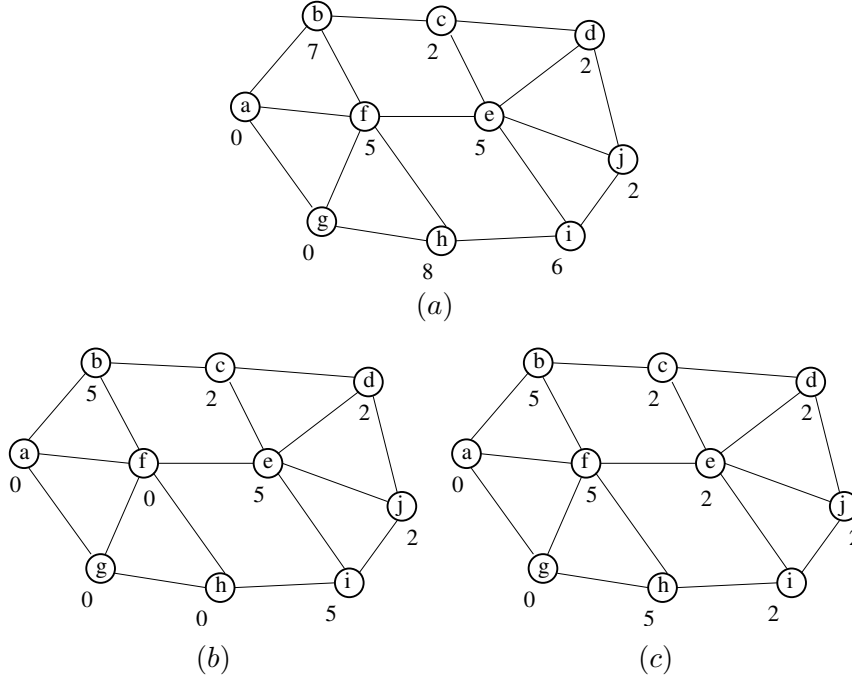
Figure 2. (a) an upstack represented by its function, (b) and (c) two topological watersheds of (a).
