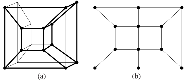
Figure 12. (a): A 1-subcomplex of the boundary of a 4-face. (b): Another view of this complex.
