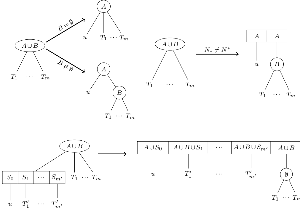
Fig. 6: Templates of a P-node
