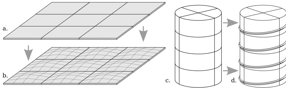
FIG. 5 – Enriched geometry of the master finite element mesh : a-b – periodic thin-walled structure, c-d – mesh of a screw with 4 turns, represented by enrichment of 16 segments with a screw function \underline{\rho}_e of the master surface \underline{\rho} .
