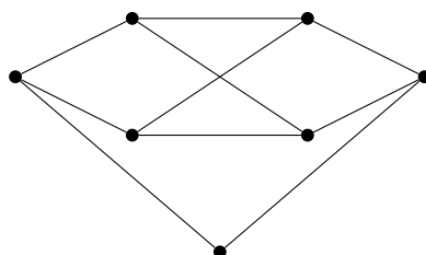
Figure 1: A graph G proposed by Erdős and Nešetřil with \chi'_s(G) = 10 .
