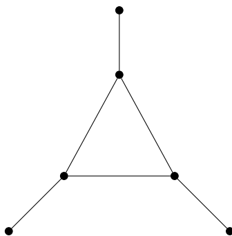
Figure 3: A graph G with mad(G) = 2 and \chi'_s(G) = 6
