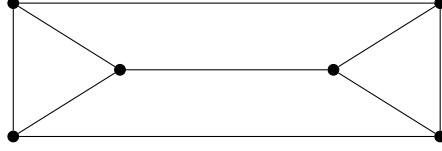
Figure 2: The prism P with \chi'_s(P) = 9
