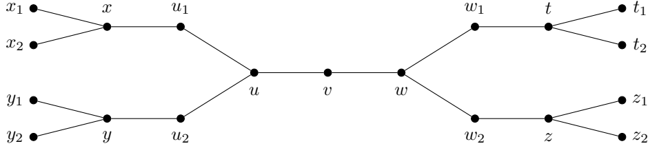
Figure 6: The configuration of Claim 2.4.
