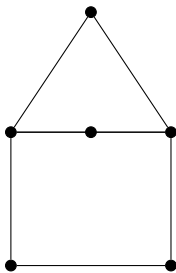
Figure 5: A graph G with \text{mad}(G) = \frac{7}{3} and \chi'_s(G) > 6
