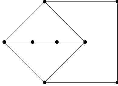
Figure 7: A graph G with \text{mad}(G) = \frac{5}{2} and \chi'_s(G) > 7
