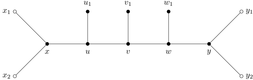
Figure 4: The configuration of Claim 1.5
