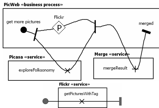
Figure 3: AoUCM: Aspect Map – Picasa Service
