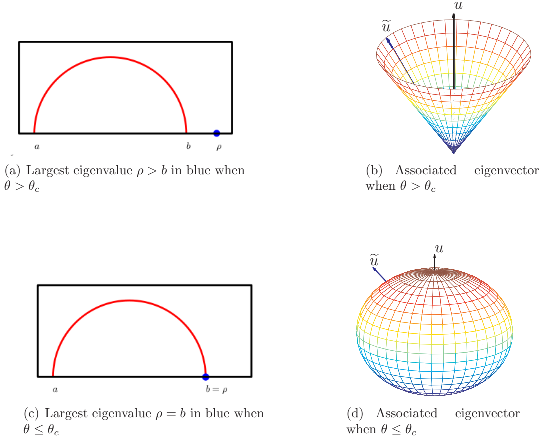
FIGURE 1. Assume that the limiting eigenvalue distribution of X_n is \mu_X with largest eigenvalue b . Consider the matrix P_n := \theta uu^* with rank r = 1 and largest eigenvalue \theta (> 0, \text{ say}) . The vector u is an n \times 1 vector chosen uniformly at random from the unit n -sphere. The largest eigenvalue of X_n + P_n will differ from b if and only if \theta is greater than some critical value \theta_c . In this event, the largest eigenvalue will be concentrated around \rho with high probability as in (a). The associated eigenvector \tilde{u} will, with high probability, lie on a cone around u as in (b). When \theta \leq \theta_c , a phase transition occurs so that with high probability, the largest eigenvalue of the sum will equal b as in (c) and the corresponding eigenvector will be uniformly distributed on the unit sphere as in (d).
