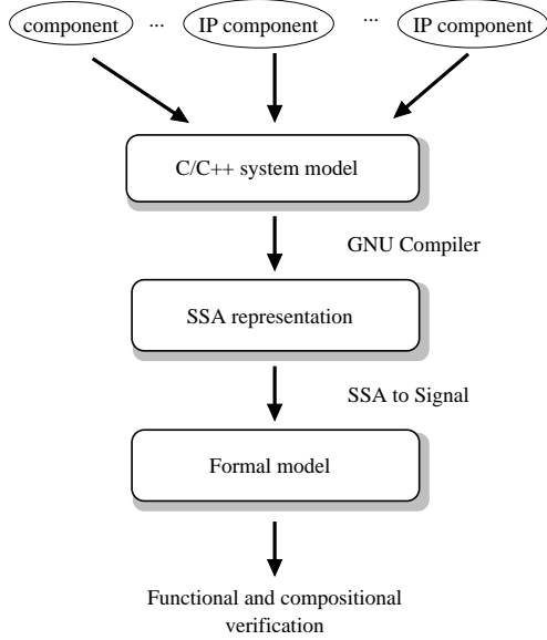
Figure 1. Our methodology
