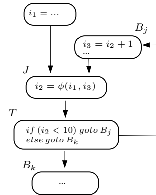
Figure 9. A Loop Statement
