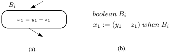
Figure 6. An SSA assignment statement (a) and its SIGNAL representation (b)
