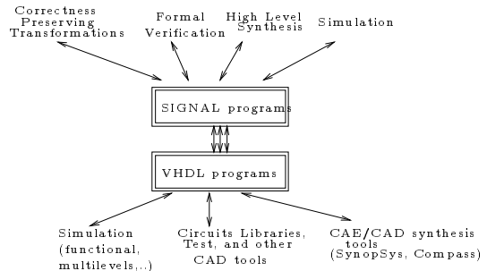
Figure 2 : VHDL/SIGNAL interface
