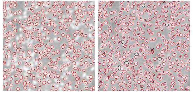
Figure 3: left: simulation step of the SEM algorithm, right: flamingo extraction using an ellipse model 387 ellipses ©INRIA ( \beta = 1000 , \gamma_d = 16.25 , s = 0.3 , d_0 = 1.33 )
