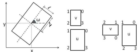
Figure 11: left: rectangle parameterization, middle: aligned rectangles, right: orthogonal rectangles.
