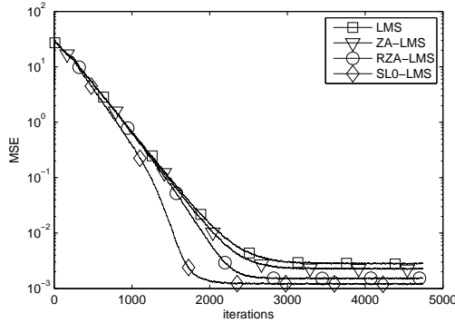
Fig. 1. Tracking and steady-state behaviors of estimation methods.
