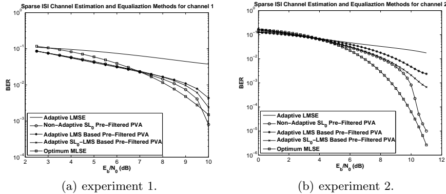
Fig. 2. Comparison of the BER-SNR curves for our estimation/equalization methods.
