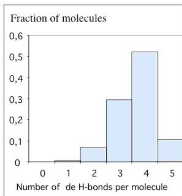
Figure 10 Numbers of water molecules (as fractions of the total number of water molecules in the liquid) that have respectively 2, 3, 4 or 5 bonds. From [7].
