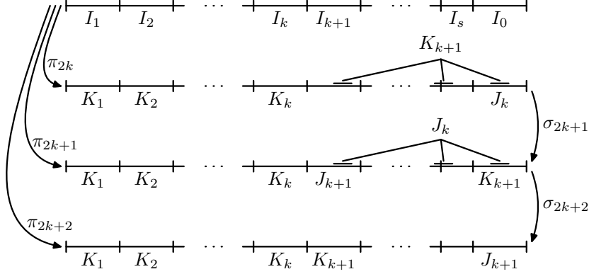
Figure 1: An illustration of the actions of the bijections \pi_{2k+1} and \pi_{2k} . The colors in K_{k+1} are not used on level 2k+1 , and the colors in J_{k+1} are not used on level 2k+2 . Moreover, \pi_{2k} and \pi agree on I_1 \cup \dots \cup I_k .
