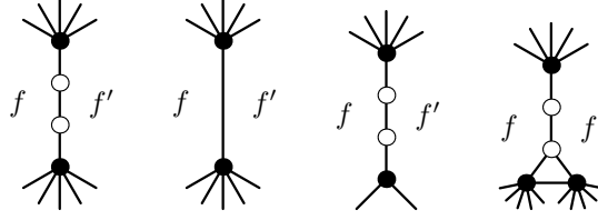
Figure 2: Examples of an (\geq 5) -face f' that is strongly adjacent to a face f ; the vertices strongly shared by f and f' are represented by empty circles. The faces f and f' also touch in the first, third and fourth example. In the second example, f' is strongly adjacent to f even if f' is a 3- or 4-face.
