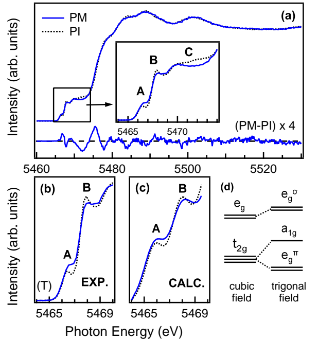
FIG. 1: (Color online) (a) V K -edge x-ray absorption spectra in (V_{1-x}Cr_x)_2O_3 , x = 0.011 powder sample measured as a function of temperature (T) in the PM (200 K, solid line) and PI (300 K, dotted line) phases by PFY XAS; below, PM-PI spectral difference; (inset) pre-edge region. (c) Calculated isotropic CI V K -edge PM and PI spectra of V_2O_3 . The spectra are compared to the T-dependent experimental data shown in the same energy window (b). (d) From LDA (starting point for our LDA+DMFT and CI calculations) we obtain that the cubic part of the ligand field splits the V d -levels in t_{2g} and e_g by 10Dq \sim 2 eV, and that the small trigonal distortion further separates the t_{2g} into a_{1g} and e_g^\pi by \Delta_{\text{trig}} \sim 0.3 eV.
