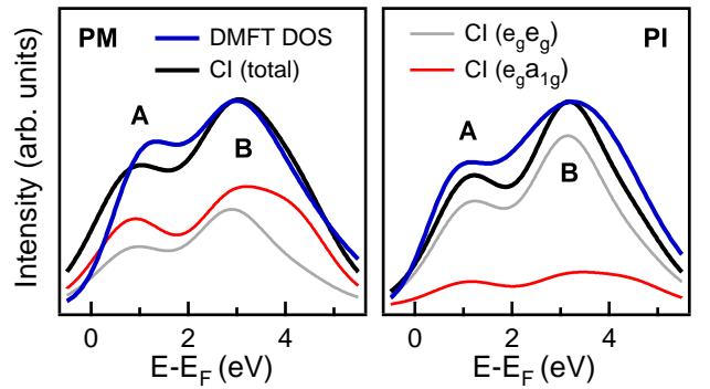
FIG. 2: (Color online) Incoherent LDA+DMFT and CI calculations in the pre-edge region; E_F is the Fermi energy. Note the similarity in the main spectral features when crossing the MIT. Also shown are the different contributions of the CI spectrum labeled accordingly to their initial state: the contribution of the (e_g^\pi, a_{1g}) \rightarrow (e_g^\pi, e_g^\pi, a_{1g}) transitions to the peak A(B) is approximately 60%(55%) in the PM phase and 20%(15%) in the PI phase.
