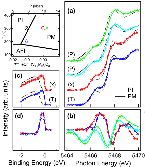
FIG. 3: (Color online) (a) V-K XAS spectra for powder samples of (V_{1-x}Cr_x)_2O_3 as a function of pressure ( \times ) [ x = 0.028 ; 5 and 7 kbar (lower curves); 5 and 11 kbar (upper curves)] (P), temperature ( \Delta ) [ x = 0.011 ; 200,300 K] (T), and doping (o) [ x = 0, 0.011 ] ( x ) (cf. points in the phase diagram; the pressure scale refers to the x = 0.028 doping). The spectral differences PM-PI ( \times 3 ) shown for the three datasets (b) demonstrate the nonequivalence between P and temperature-doping. The x - T equivalence is confirmed by the photoemission spectra ( h\nu = 9 eV) (c) and their spectral differences (d) (from Ref. [15]).
