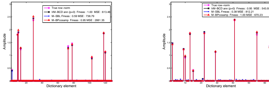
Fig. 7. Examples of estimated row-norm using 3 different algorithms. left) M = 128, N = 64, k = 10 and L = 3 . right) M = 64, N = 64, k = 10 and L = 3 . Here, we want to illustrate cases where a “good” sparsity recovery does not necessary lead to low mean-square error.
