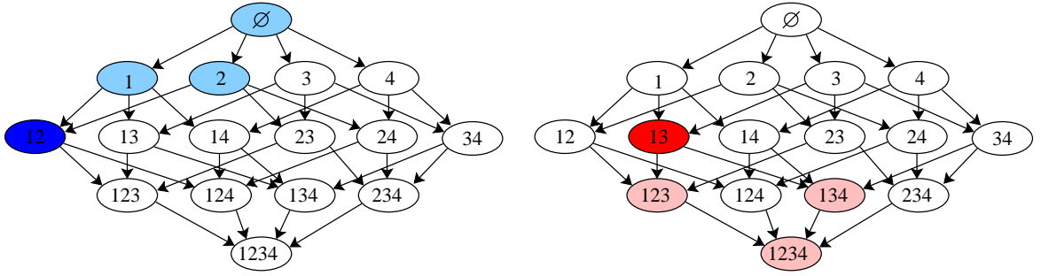
Figure 5: Directed acyclic graph of subsets of size 4: (left) a vertex (dark blue) with its ancestors (light blue), (right) a vertex (dark red) with its descendants (light red). By zeroing out weight vectors associated with descendants of several nodes, we always obtained a set of non-zero weights which contains all of its own ancestors (i.e., the set of non-zero weights is equal to its hull).
