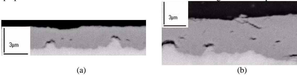
Fig. 6 : Cross-sectional views of oxide layers grown on ZrNbO at 530^\circ\text{C} ( P_{\text{H}_2\text{O}} = 13\text{hPa} , P_{\text{H}_2} = 10\text{hPa} ) : X \approx 3.5\ \mu\text{m} (a) and X \approx 6\ \mu\text{m} (b).
