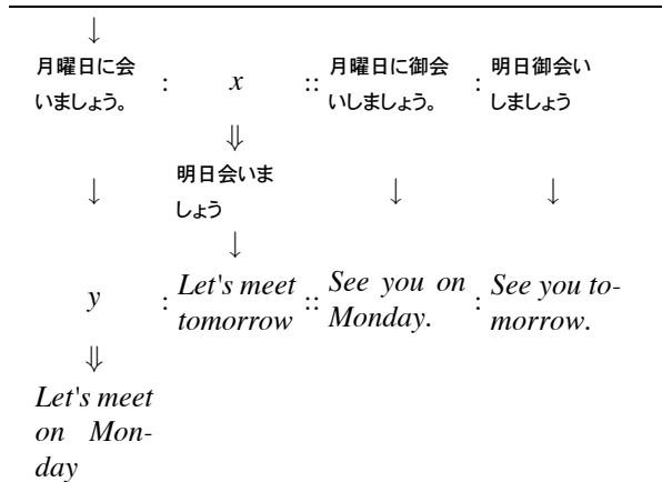
Figure 1: A sketch of the translation principle by corresponding proportional analogies, illustrated on actual data from IWSLT 2007. The Japanese sentence on the left is the input. The Japanese strings on the same line are from the training data or the alignment results. Solving the Japanese equation yields the Japanese string in the middle, which, incidentally, belongs to the alignment data. From the corresponding translations, a candidate translation for the input is obtained in place of y .
