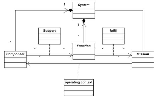
Figure 2 – UML Class diagram of the conceptual view of the structural model
