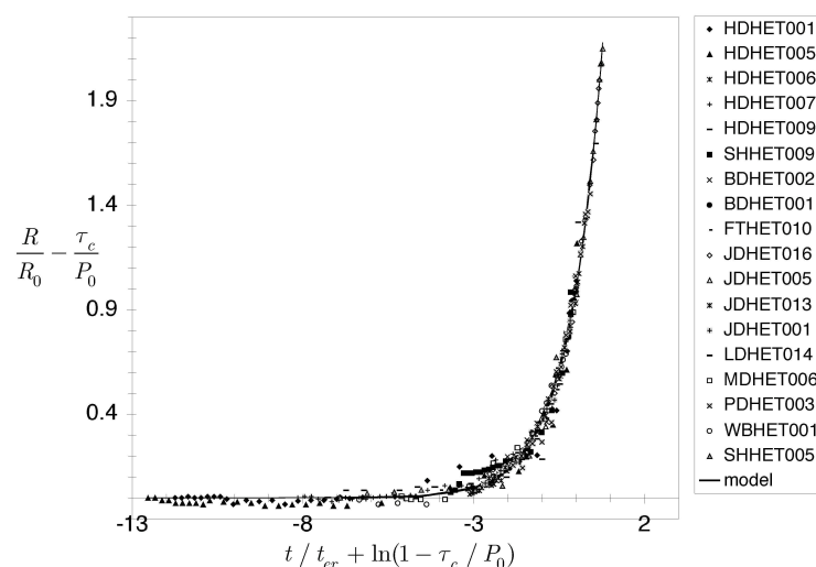
FIG. 2 – Hole Erosion Tests (symbols) versus scaling law (continuous lines). Dimensionless radius is shown as a function of dimensionless scaling time.
