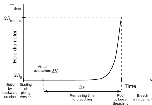
FIG. 4 – Evaluation of remaining time to breaching using the scaling law
