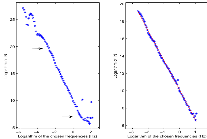
Fig. 10. The log-log graph of the variance of wavelet coefficients relating to the HR series observed in the middle of the exercise (Ath5)
