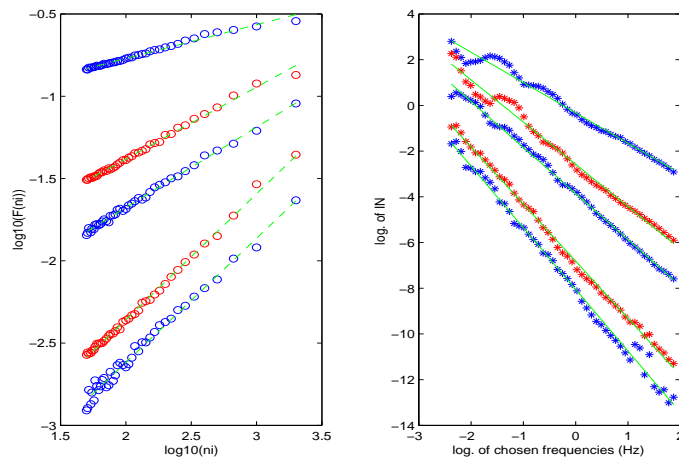
Fig. 6. Results of the DFA method and wavelet analysis applied to a path of a discretized FGN for different values of H = 0.2, 0.4, 0.5, 0.7, 0.8 , with N = 10000
