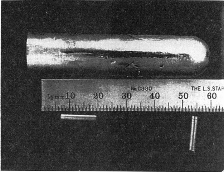
Figure 1. Photo of Zr base metallic glass ingot and projectiles.
