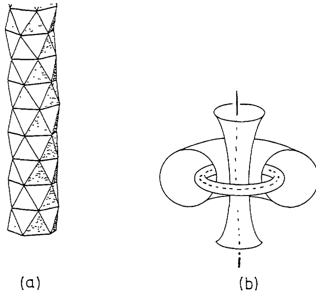
Fig. 3. — A column obtained by piling up pentagonal antiprisms, it can be decomposed into a tetrahedral packing (a), « flat » representation of the spherical torus at midway between the two interlaced organization of the circles and the two tori organized like in (a); in this representation one circle appears like a straight line, but in S^3 both circles have the same radius (b).
