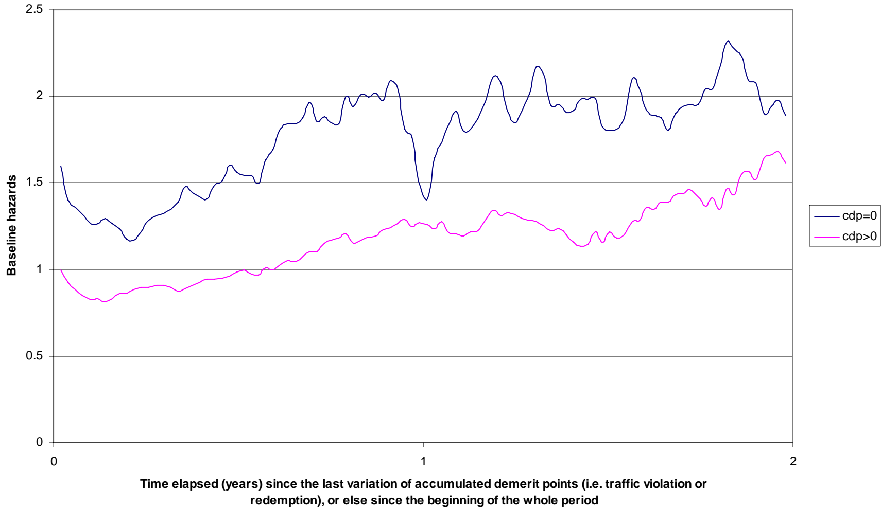
Figure 3. Baseline hazard functions for traffic violation risk, stratification by accumulated demerit points (cdp) in the last two years (strata cdp=0 and cdp>0) One month moving average, vertical unit=initial value for the stratum defined by cdp>0
