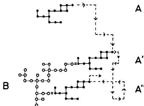
Fig. 1. — Sketch of diffusion process. Two clusters diffuse (dotted line, one cluster held fixed) until they touch (A \rightarrow A'). A bond is formed with probability p . If not, the diffusion continues (no overlap of the clusters) until the clusters touch again (A' \rightarrow A''), etc...
