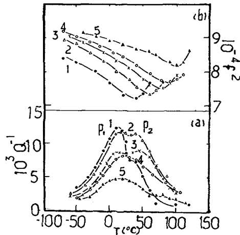
Fig. 7. Internal friction and elastic modulus of specimen S4 (Mn 56.16/Cu 40.25/Al 3.59) aged at 450°C for various times. Curves 1-5 correspond to ageing time of 0.5, 1, 2, 4, and 9 h. f = 1 kHz, A_\varepsilon = 5.2 \times 10^{-6} , \dot{T} = 1^\circ\text{C}/\text{min} with ascending temperatures.
