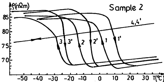
Fig.1. Effect of heat treatments on the e.r. 180 ^{\circ}C , which does not show relaxation character. 1,1'- 800 ^{\circ}C/1h Q(RT,w); 2,2'- 1,1' + 130 ^{\circ}C/1h Q(RT,w); 3,3'- 2,2' + 180 ^{\circ}C/1h Q(RT,w); 4,4'- 3,3' + 216 ^{\circ}C/1h Q(RT,w).
