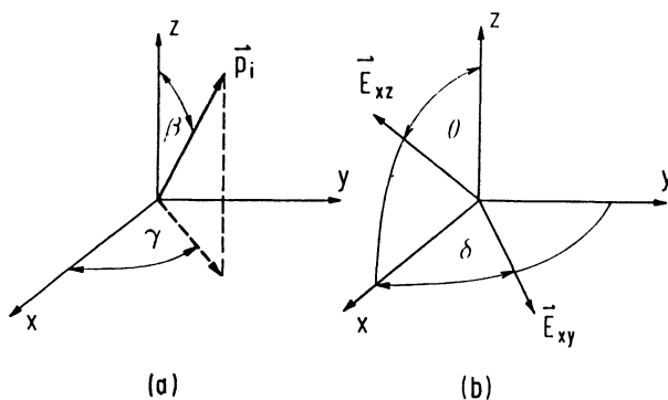
Fig. 2. — (a) shows orientation of the induced molecular dipole moment \mathbf{p}_i in the laboratory frame with z axis normal to the smectic layers and y axis parallel to ferroelectric polarization in the S_C^* phase. (b) defines the angles \delta and \theta that measure the orientation of the optical electric field in the x - y and x - z planes respectively.
