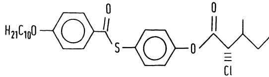
Fig. 1. — Molecule of the \overline{10} .S.C1Isoleu liquid crystal.
