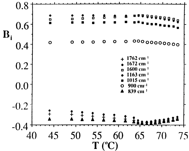
Fig. 3. — Temperature dependence of the order parameters B_i for the seven molecular dipole moments associated with different molecular vibrations. Center frequencies are marked in the figure. Phase transition temperatures on cooling are T_{AI} = 74^\circ\text{C} and T_{CA} = 66^\circ\text{C} .
