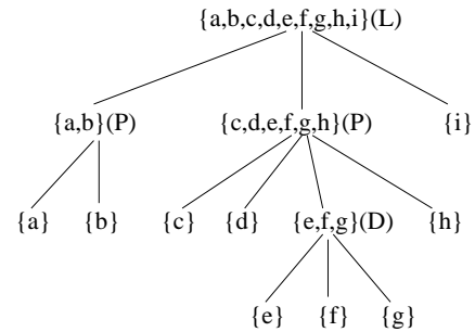
Figure 2: The modular decomposition represents the modules of a graph with an ordered tree whose nodes are subsets of V . Each internal node is labeled linear (L), prime (P), or degenerate (D). A subset of the vertices is a module iff it is a node of the tree, the union of a set of children of a degenerate node, or the union of a set of children of a linear node that is consecutive in the left-to-right order of its children. The modules of the depicted graph that are not nodes of the tree are unions of children of \{e, f, g\} , namely, \{e, f\} , \{e, g\} , and \{f, g\} , and unions of consecutive children of \{a, b, c, d, e, f, g, h, i\} , namely, \{a, b, c, d, e, f, g, h\} and \{c, d, e, f, g, h, i\} . To represent the decomposition, it is not necessary to label internal nodes with the set that they correspond to, as this is given by the union of leaf descendants of the node.
