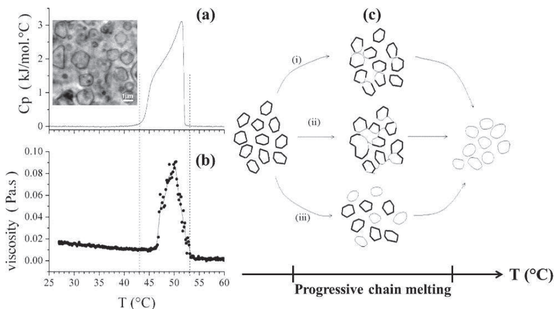
Figure 3: (a) Heat capacity scan obtained by DSC showing the progressive chain melting occurring from 43°C to 53°C leading to the transition between faceted vesicles to unilamellar vesicles. (b) Evolution of the bulk viscosity as a function of temperature measured at 6.28 \text{ rad s}^{-1} of catanionic vesicles ( \Phi = 0.1 \text{ wt}\% ). (c) Schematic showing the possible intermediate states between faceted polyhedra and unilamellar vesicles occurring during the chain melting and at the origin of the rheological behavior. The thick lines symbolize the ordered chains, while the fine, curved lines stand for the disordered chains. Adapted from [43] with permission. Copyright 2004 American Chemical Society.
