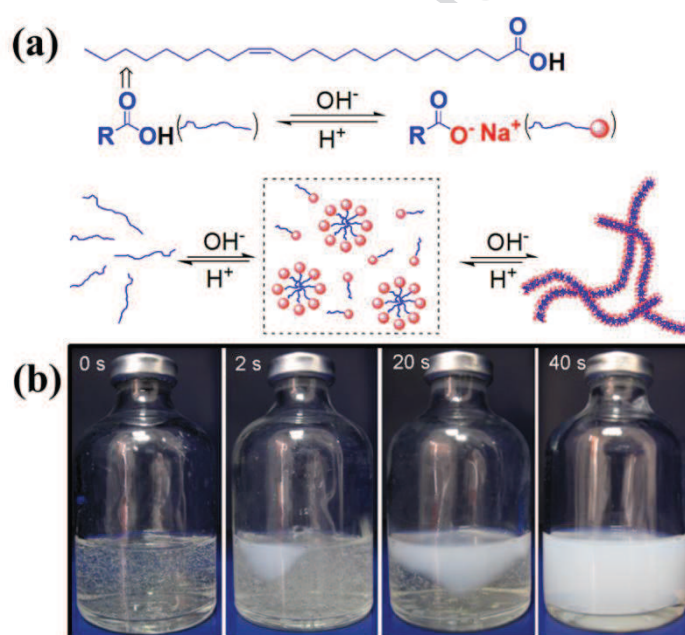
Figure 1: (a) Schematic illustrating the chemical principles of the pH-switchable wormlike micelles obtained with the erucic acid. (b) Snapshots showing the evolution of the 100mM erucic acid solution as a function of the carbon dioxide bubbling time. Reprinted and adapted from [35, 36] with permission.
