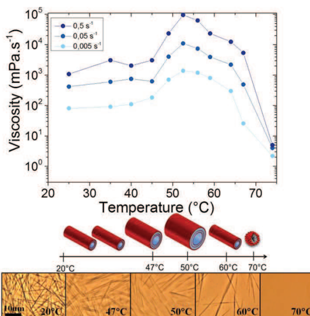
Figure 2: Evolution of the viscosity of the 12-HSA tubes solution as a function of temperature for three different shear rates. The 12-HSA tubes structural evolution occurring in bulk with temperature is illustrated by the schematic and the corresponding pictures obtained by phase contrast microscopy. Adapted from [46, 47] with permission from American Chemical Society and The Royal Society of Chemistry. Copyright 2011 American Chemical Society.
