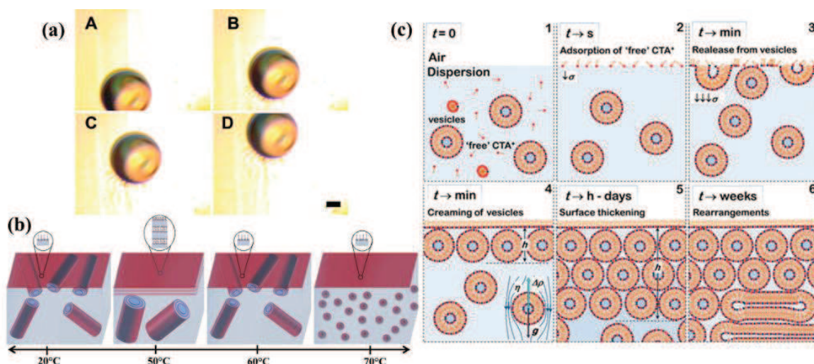
Figure 4: (a) Self-propelling droplet motion observed by phase contrast microscopy (A–D). The droplet moves from the bottom to the top and each frame is captured at 2 s intervals. The scale bar is 100 \mu\text{m} . Reproduced from [54] with permission. Copyright 2007 American Chemical Society. (b) Schematic illustration of the structural and dynamic properties of the 12-HSA tubes at the air/water interface with temperature determined by neutron reflectivity experiments. Reproduced from [4] with permission. Copyright 2011 American Chemical Society. (c) Schematic illustrating the adsorption phenomenon occurring in cationic vesicles obtained with myristic acid with time. Reproduced from [6] with permission. Copyright 2013 American Chemical Society.
