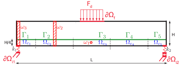
Fig. 5 2D concrete beam with a horizontal steel bar, with domains of interest \omega_1 , \omega_2 and \omega_3 .
