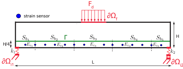
Fig. 6 Instrumentation of the beam with 14 strain sensors.
