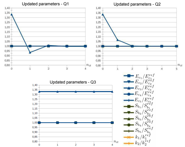
Fig. 7 Updated beam parameters at each iteration of the updating goal-oriented approach for quantities of interest Q_1 , Q_2 , and Q_3 .
