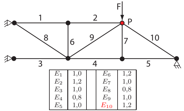
Fig. 2 Considered trussed structure (left) and reference values for the material parameters (right).
