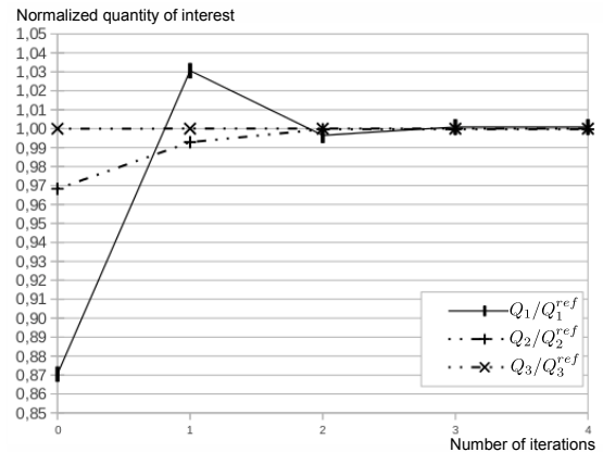
Fig. 8 Ratio between the updated and the reference values of the quantity of interest at each iteration of the updating goal-oriented approach for Q_1 , Q_2 and Q_3 .
