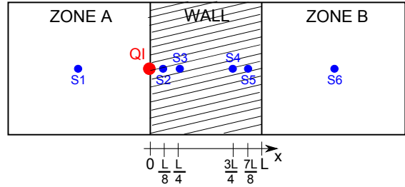
Fig. 9 Geometry of the unsteady thermal problem with two zones and one wall. S_i denotes the i^{th} temperature sensor and QI the quantity of interest.
