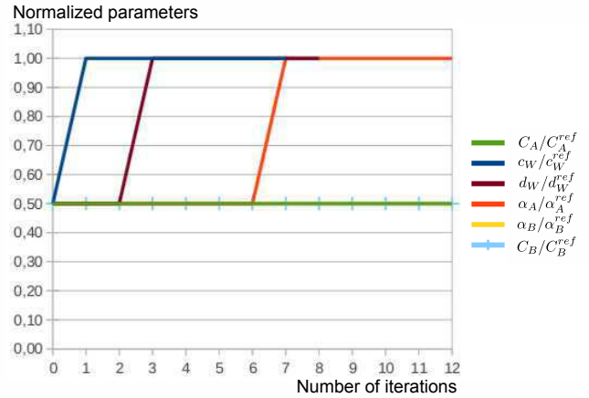
Fig. 13 Updated parameters \mathbf{p} with the goal-oriented calibration technique - Case of non-corrupted sensor outputs.
