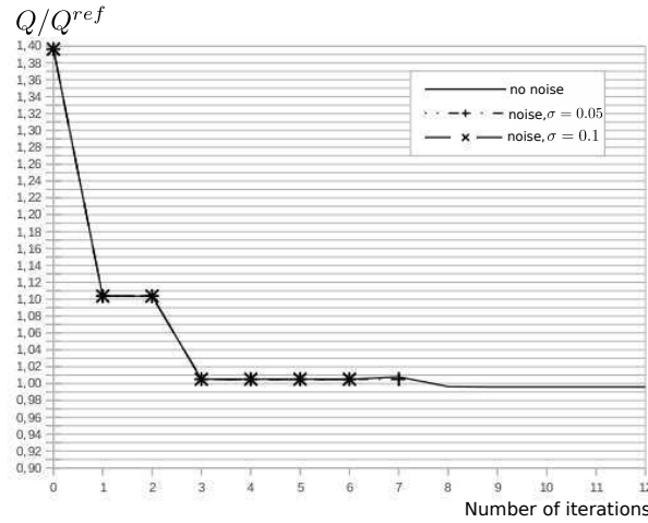
Fig. 12 Ratio of the updated quantity of interest and the reference quantity of interest at each iteration, obtained with the goal-oriented calibration technique.
