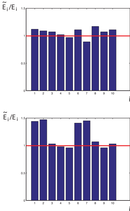
Fig. 4 Ratio E_i^*/E_i after iteration 10 in the updating process, for classical updating (left) and updating dedicated to Q (right).
