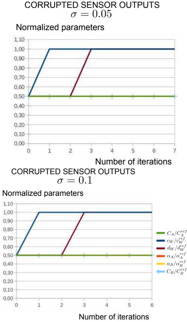
Fig. 15 Parameters \mathbf{p} updated with the goal-oriented method - Case of corrupted sensor outputs.
