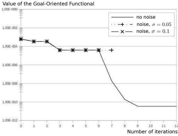
Fig. 11 Goal-oriented functional at each iteration.
