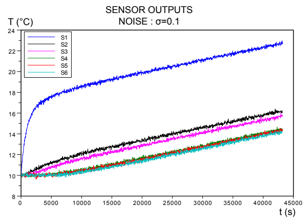
Fig. 14 Corrupted sensor outputs.
