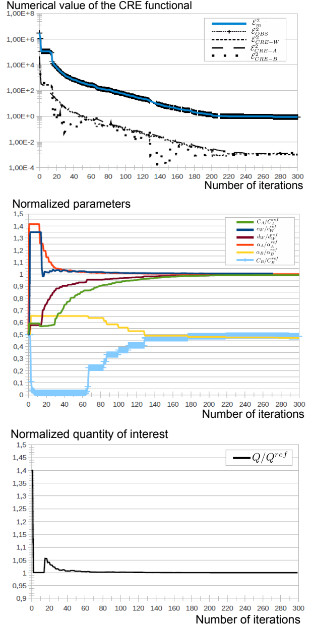
Fig. 10 Modified constitutive relation error, normalized parameters and ratio between the updated quantity of interest and the reference quantity of interest at each iteration - Case of non-corrupted sensor outputs.
