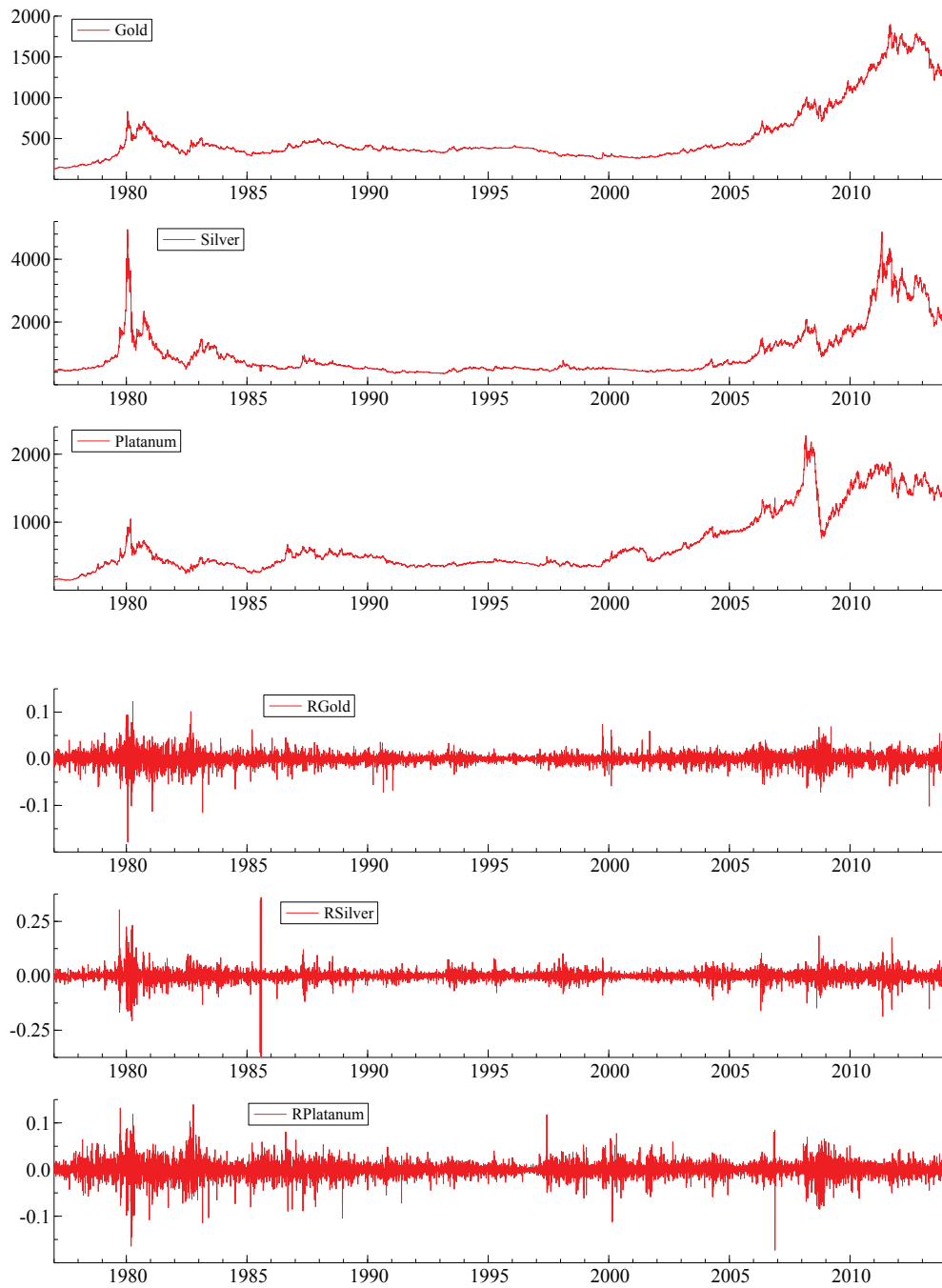
Figure 1: Time Plots of Precious metal prices and returns: Daily from 1977 to 2013
