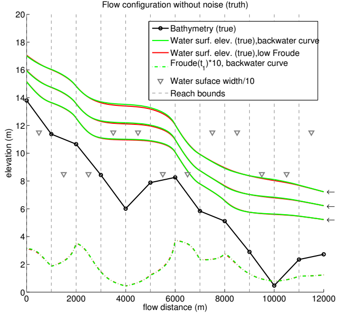
Figure 4: forward models on generic river test case configuration: permanent flows at three times without noise. Dashed lines correspond to Froude variability at t_1 .
