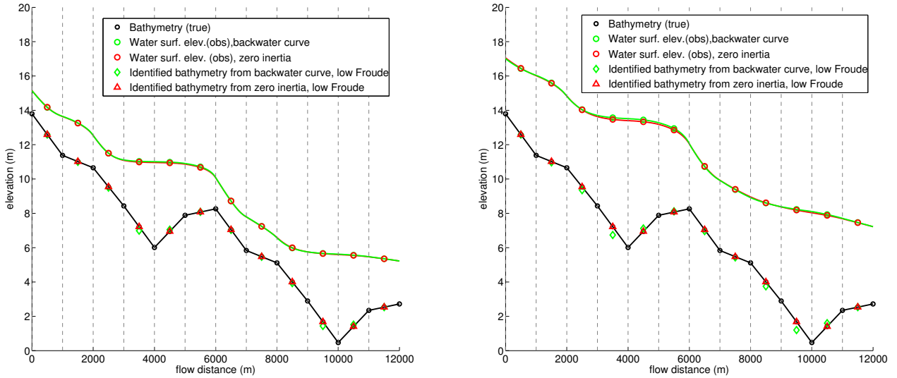
Figure 8: Bathymetry identification for the synthetic test case with low Froude model and “perfect observations”, (left) t = t_1 , (right) t = t_3 . Continuous green and red line represent the true water surfaces calculated with the ODE solver for the backwater curve and the low Froude model. Flow features are summed up in Table 1 and Figure 4..
