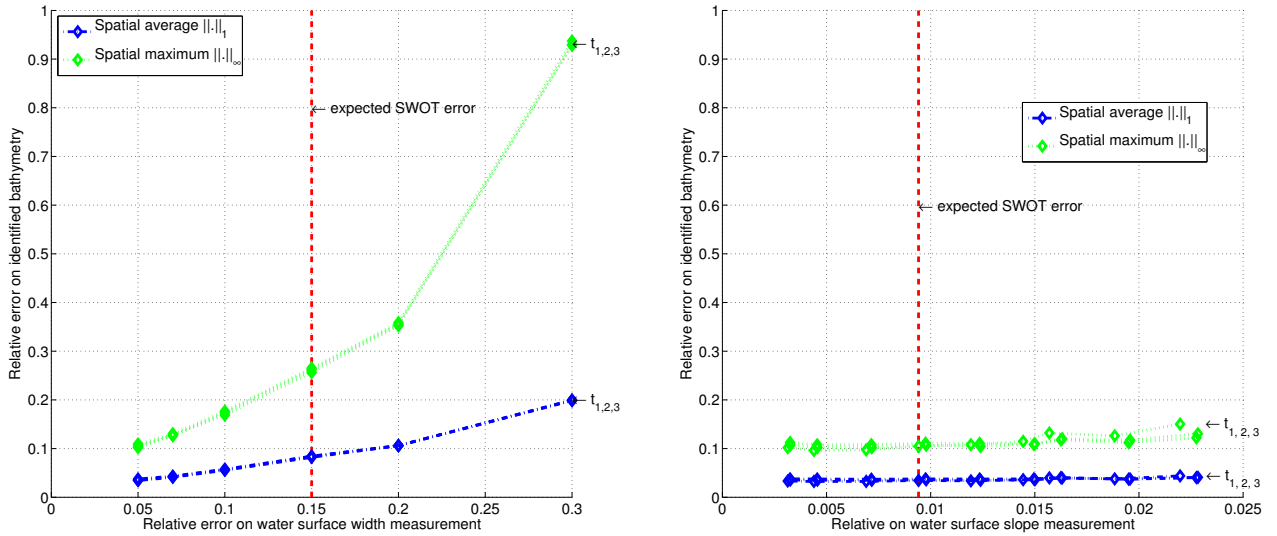
Figure 10: Sensitivity of the the identified bathymetry A_0 to measurement errors. Flow features are summed up in Table 1 and Figure 4.
