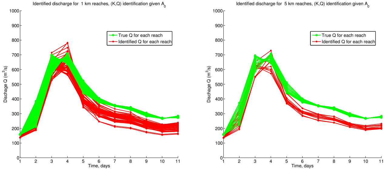
Figure 15: Identification of (K, Q) given A_0 for the 9 th to the 20 th of November 2004 for each reach: identified discharge along the flow distance for the Garonne River; first guess is (K_b, Q_b^1, Q_b^2, Q_b^3) = (40, 400, 400, 400) with SWOT like observations, (left) for 1km reaches and (right) for 5km reaches (hence 5 observation values are averaged for each reach). In both cases spatially averaged RMSE = 14.3\% on discharge and the relative error on the roughness K is +36%. Each set of curve represents the spreading of reach behaviors along the flow distance.
