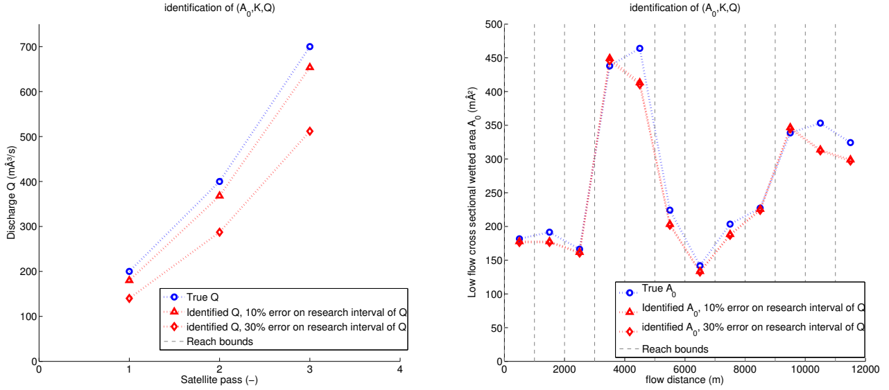
Figure 6: Results obtained while performing the triplet (A_0, K, Q) identification : (left) the discharge Q , (right) the base-flow cross sectional area A_0 , and the roughness K = 20.1 \text{ m}^{1/3} \cdot \text{s}^{-1} (the truth being K_t = 20 \text{ m}^{1/3} \cdot \text{s}^{-1} ). Observations with SWOT like errors. Flow features are summed up in Table 1 and Figure 4.
