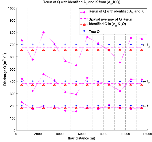
Figure 7: Re-computation of the discharge Q given A_0 and K identified at 2.7% and 1.1% relative errors (using the triplet inversion method with observations SWOT like errors amplitudes).
