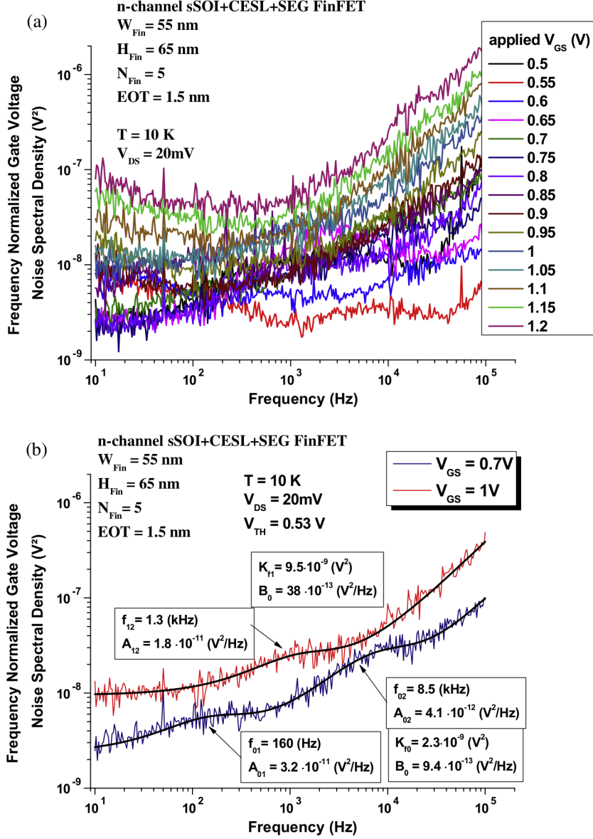
Fig. 4. Typical frequency normalized gate voltage noise spectral density for a strained device at 10 K for L_C = 0.2 \mu\text{m} . (a) For all applied gate voltages; (b) Comparison between experimental noise spectra and model of equation 1 (black lines). White noise, flicker noise and Lorentzian contributions are considered to obtain the best agreement between the experimental noise spectra and model.
