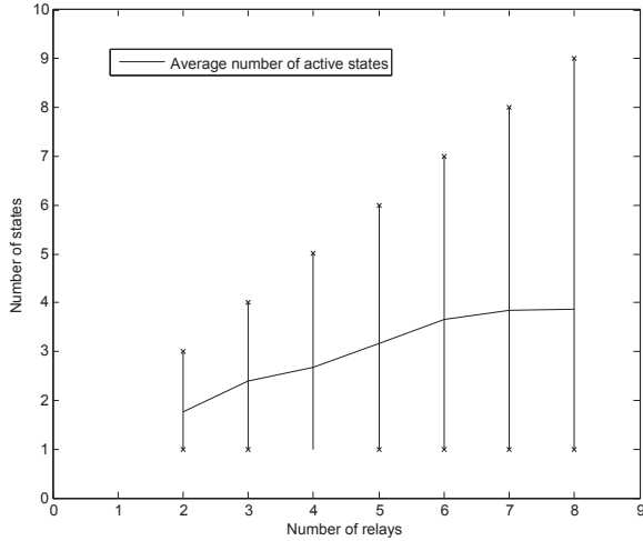
Fig. 1. Average, minimum and maximum number of active states to characterize the capacity of a HD relay network.
