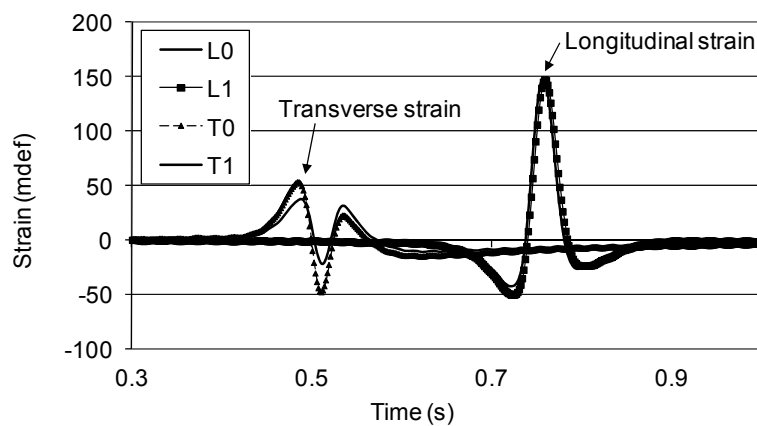
Figure 12. Signals of longitudinal and transverse strain gages under the center of a dual wheel, at 21°C, 53 000 loads, V=43\text{km/h}
