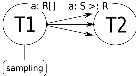
Figure 5: Exploration transition.
